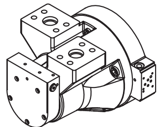
CS TYPE SHUTTLE ENDCAP ON F4 & FM4 ASSEMBLIES ONLY
