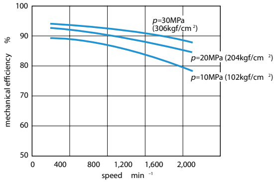
◆ Mechanical efficiency (%)
