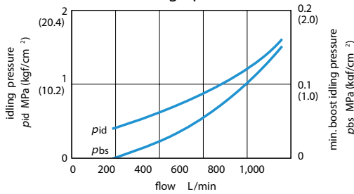
◆ Idle & boost-graph
