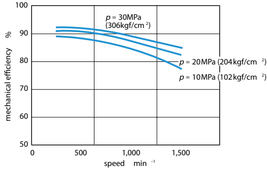
◆ Mechanical efficiency (%)
