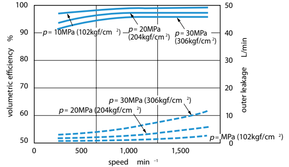
◆ Volumetric efficiency
