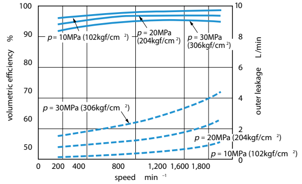
◆ Volumetric efficiency
