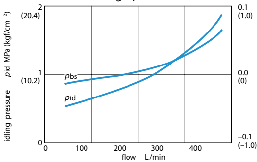
◆ Idle & boost-graph
