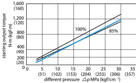
◆ Idle & boost-graph
